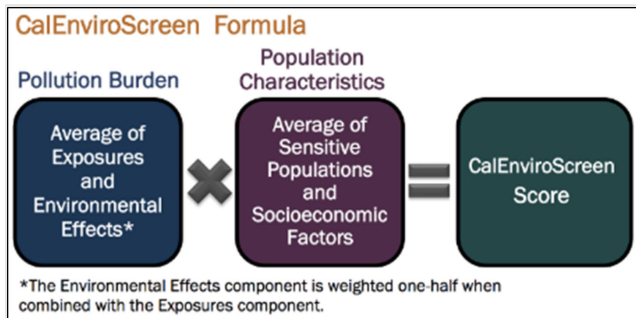
Figure 8-4: CalEnviroScreen Formula
