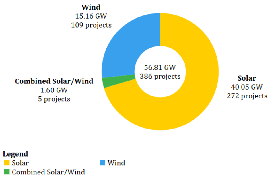
Figure 3-1: RTO Renewable Resource Queue (PJM & MISO, As of July 2025)
