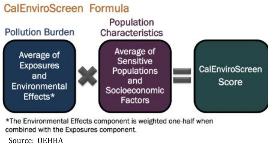
Figure 8-7: CalEnviroScreen Formula
